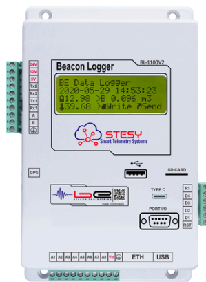
Beacon Data Logger BL-1100 Series
